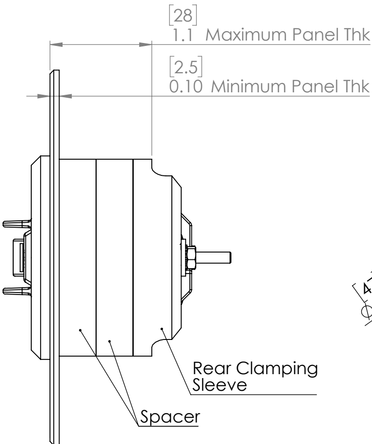
Panel Thickness Guide for Rear-Mount
