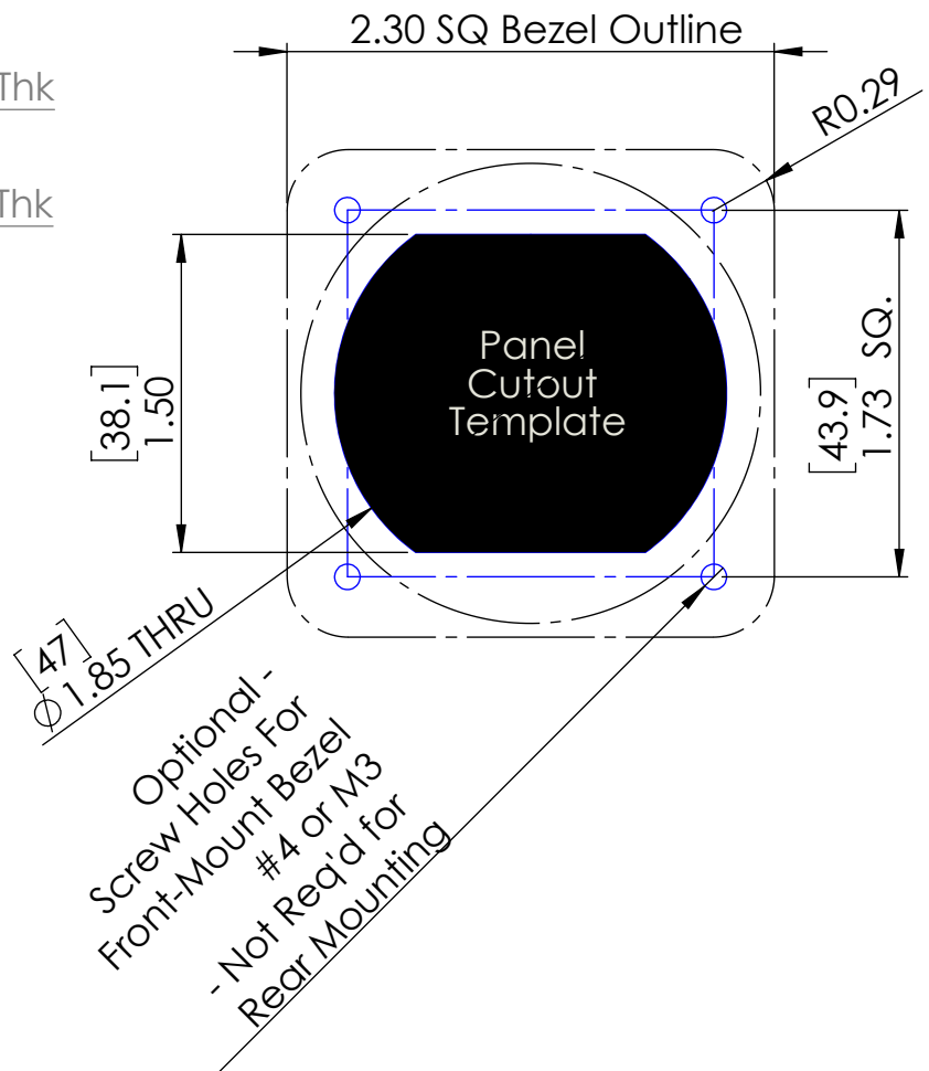
Perimeter and Screw Pattern for Front-Mount Bezel
